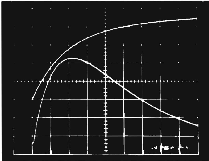
Fig. 1. Typical response curves at 2 \mu\text{s}/\text{cm} . The upper trace is V(t) at 0.2 \text{ V}/\text{cm} ; the lower trace is I(t) at 5 \mu\text{amp}/\text{cm} .
