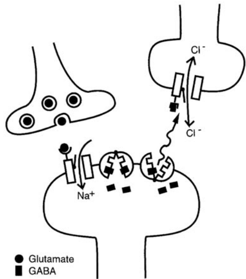
FIG. 1. Reverse uptake and volume diffusion of GABA (Atwell et al. , 1993). Glutamate is released by a presynaptic neuron and stimulates its receptors on either glial or neuronal cells, resulting in an \text{Na}^+ influx. The increased intracellular \text{Na}^+ causes GABA uptake carriers (which normally couple the influx of GABA and \text{Na}^+ ) on the postsynaptic cell to operate in reverse and extrude GABA from intracellular stores. The extracellular GABA can then diffuse and affect other cells having appropriate receptors.
